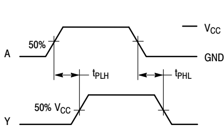
Figure 3. Switching Waveforms
