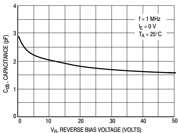
Figure 4. Output Capacitance
