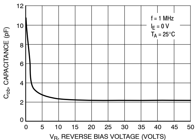
Figure 34. Output Capacitance
