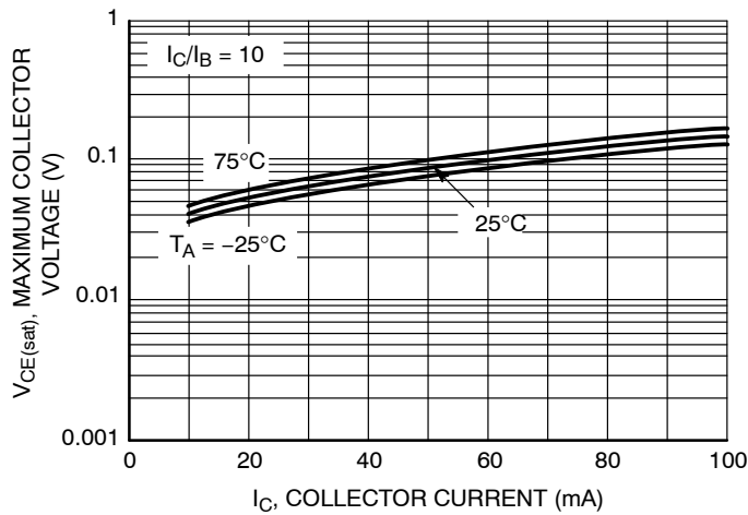
Figure 59. V_{CE(sat)} vs. I_C
