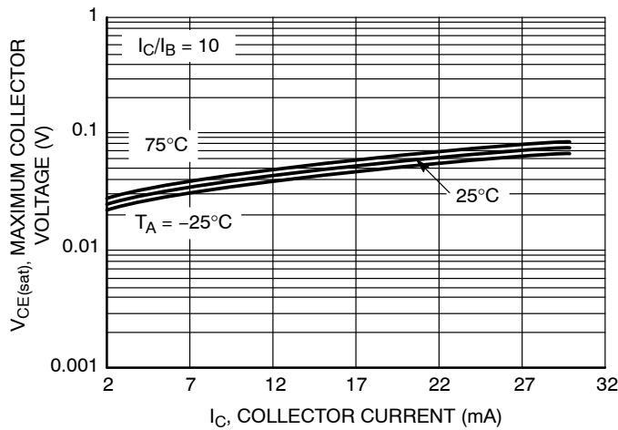
Figure 52. V_{CE(sat)} vs. I_C
