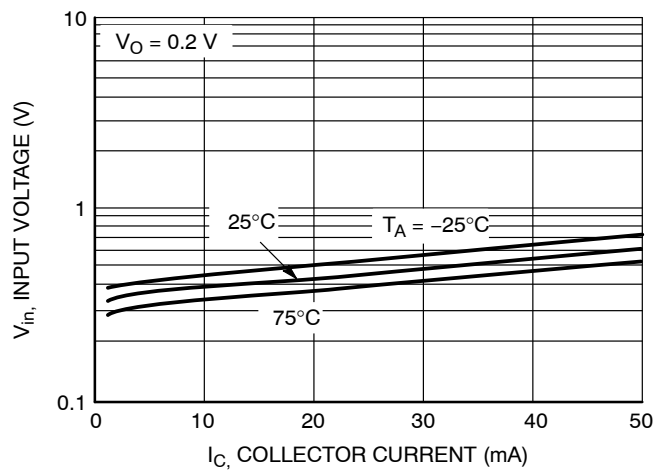
Figure 63. Input Voltage vs. Output Current
