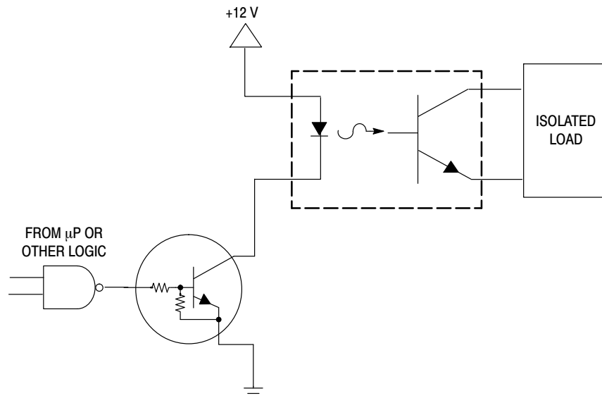
Figure 64. Level Shifter: Connects 12 or 24 Volt Circuits to Logic
