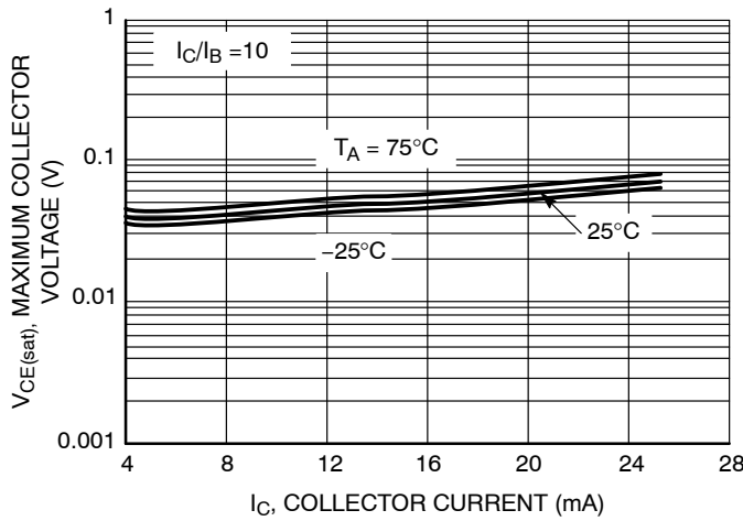
Figure 47. V_{CE(sat)} vs. I_C
