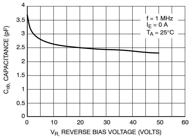
Figure 54. Output Capacitance
