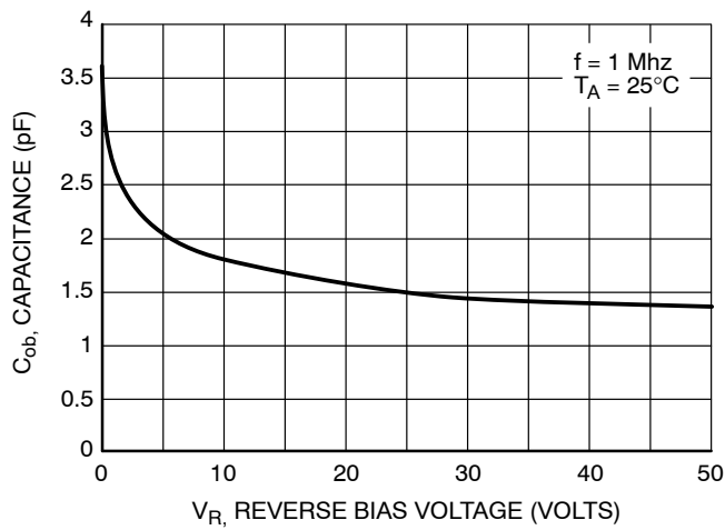
Figure 61. Output Capacitance
