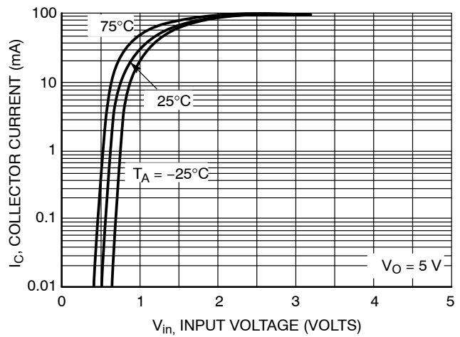
Figure 62. Output Current vs. Input Voltage
