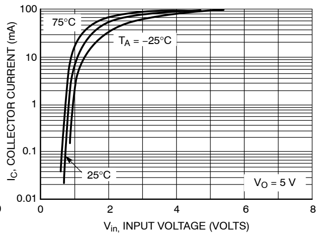
Figure 55. Output Current vs. Input Voltage
