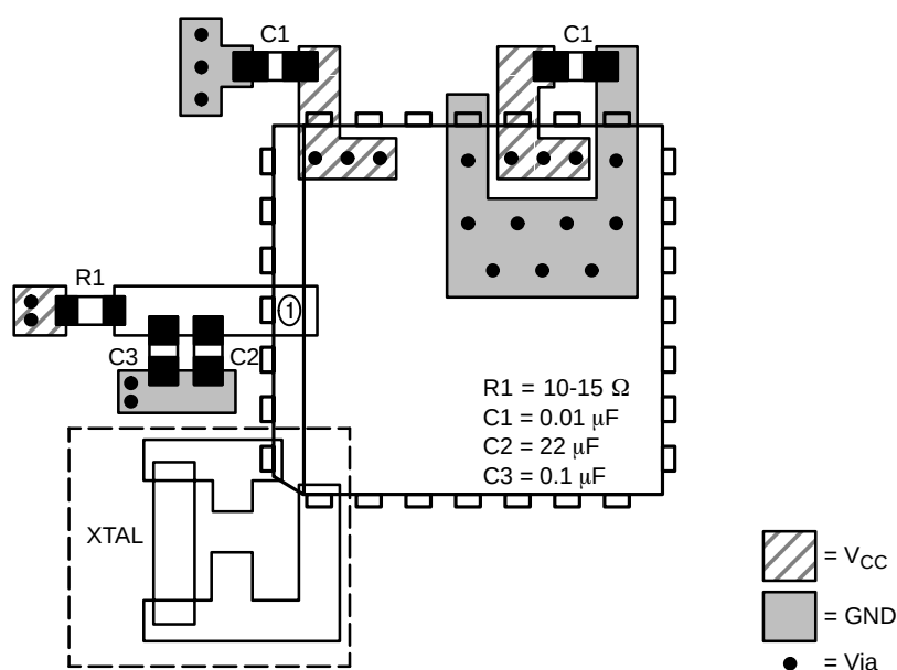
Figure 8. PCB Board Layout for NBC12430 (28 PLCC)
