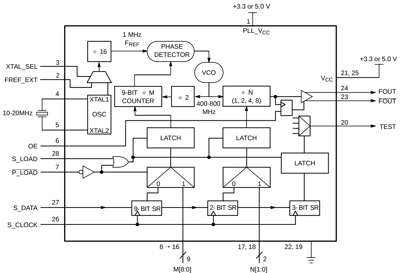
Figure 1. NBC12430 Block Diagram (28-Lead PLLC)
