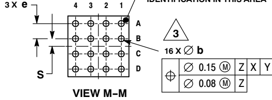
VIEW M-M
