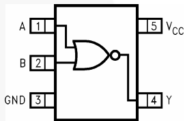
Figure 2. SC70 and SOT23 (Top View)
