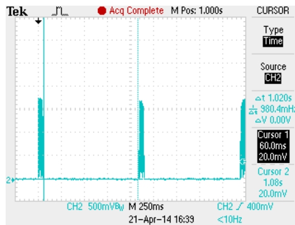
Figure 15. Current Pulses during Shorted Output
