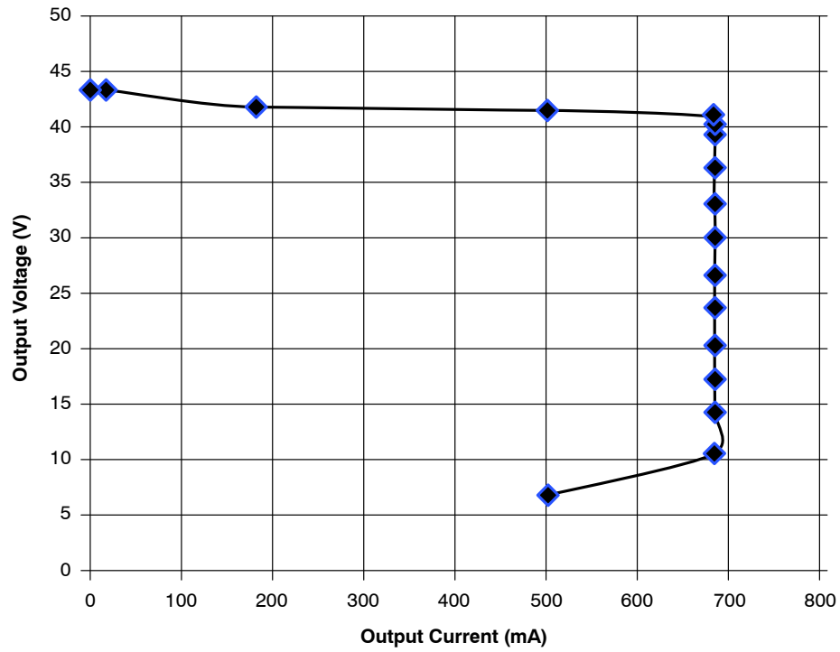
Figure 11. Load Regulation
