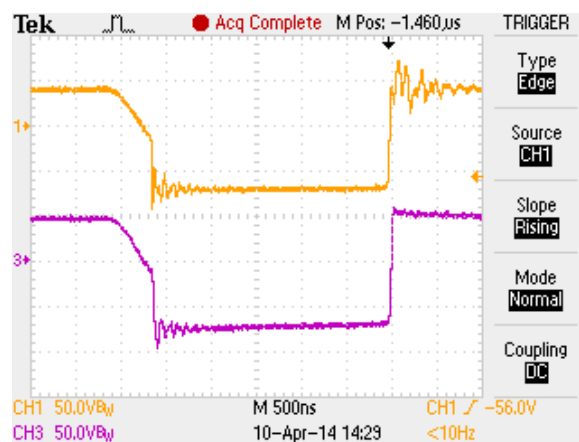
Figure 13. Bias Winding Ringing Compared to Secondary Winding Waveform
