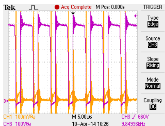
Figure 7. Drain Voltage and Current at 305 V ac Input
