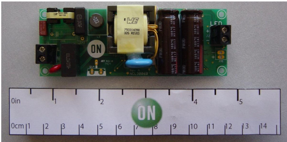
Figure 1. NCL30060G Evaluation Board (Top Side)
