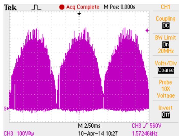
Figure 8. Drain Voltage at 230 V ac with Slower Scan
