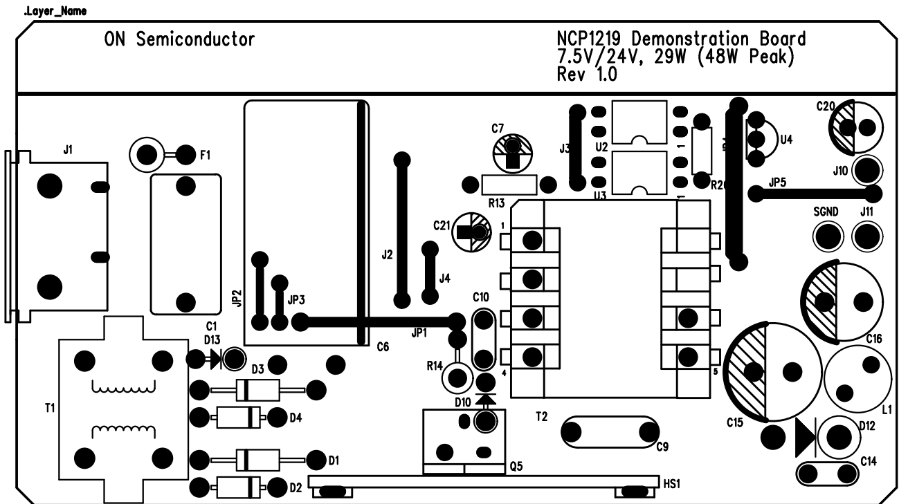
Figure 30. Layer 1 (Top)
