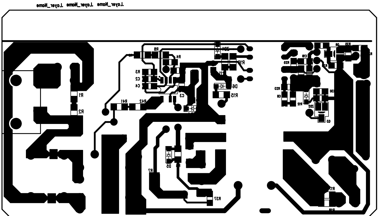
Figure 31. Layer 2 (Bottom)
