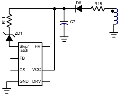
Figure 25. Primary Overvoltage Protection Circuit
