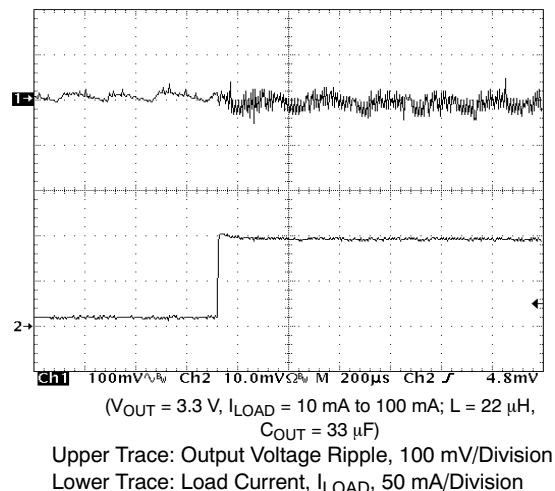
Figure 24. Load Transient Response for V_{IN} = 1.8 V
