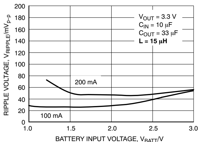
Figure 18. Output Ripple Voltage vs. Battery Input Voltage
