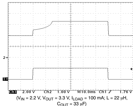
Upper Trace: Output Voltage Waveform, 2.0 V/Division Lower Trace: Shutdown Pin Waveform, 1.0 V/Division
