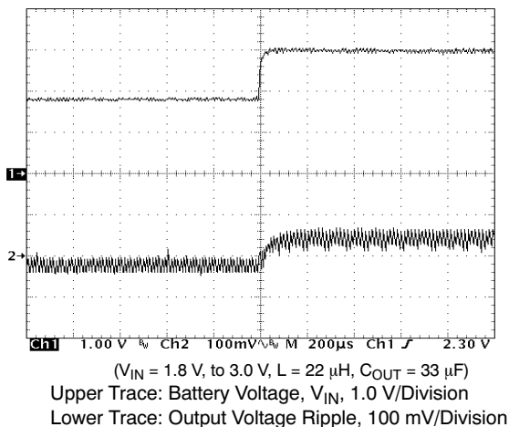
Figure 23. Line Transient Response for V_{OUT} = 3.3 V
