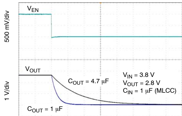
Figure 51. Enable Turn-off
