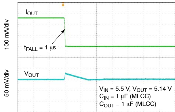
Figure 49. Load Transient Response – 250 mA to 1 mA – V_{OUT} = 5.14 V
