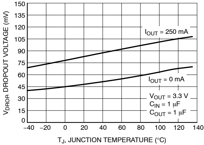
Figure 24. Dropout Voltage vs. Temperature— V_{\text{OUT}} = 3.3\text{ V}
