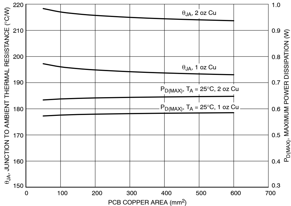
Figure 54. \theta_{JA} and P_D (MAX) vs. Copper Area (XDFN44)
