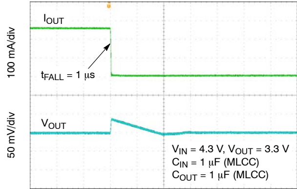
Figure 47. Load Transient Response – 250 mA to 1 mA – V_{OUT} = 3.3 V
