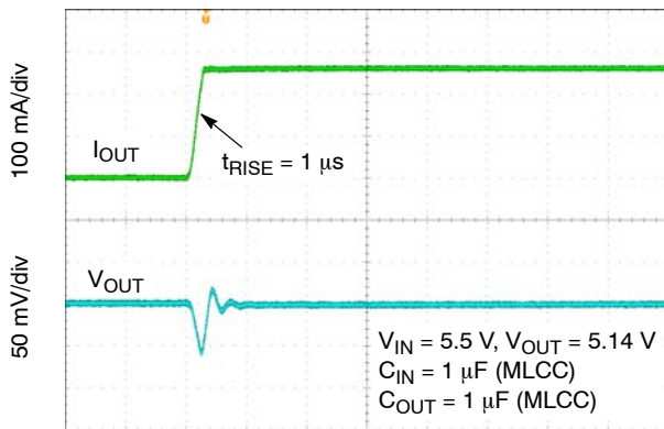
Figure 48. Load Transient Response – 1 mA to 250 mA – V_{OUT} = 5.14 V
