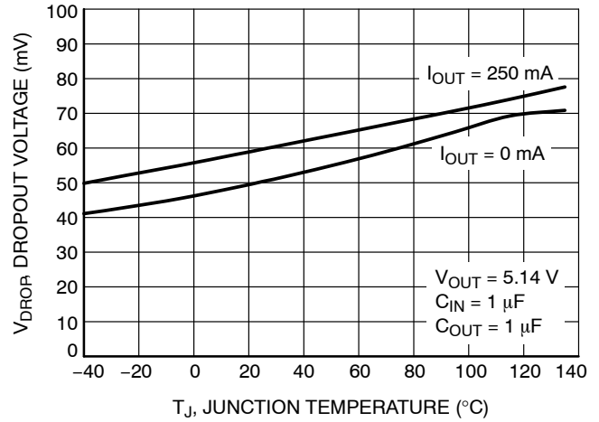
Figure 25. Dropout Voltage vs. Temperature— V_{\text{OUT}} = 5.14\text{ V}
