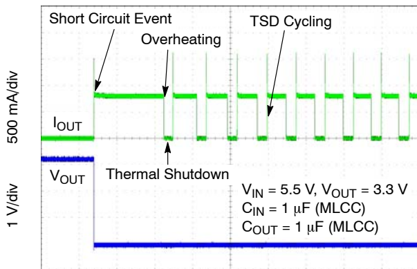
Figure 50. Short Circuit and Thermal Shutdown
