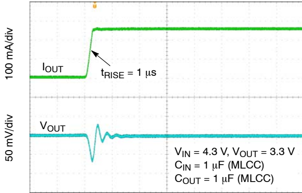
Figure 46. Load Transient Response – 1 mA to 250 mA – V_{OUT} = 3.3 V
