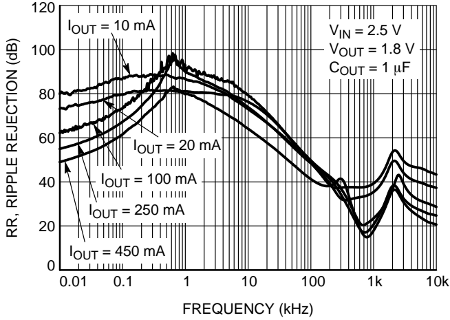
Figure 31. Power Supply Rejection Ratio, V_{OUT} = 1.8\text{ V}
