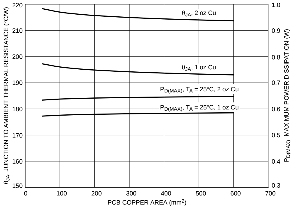
Figure 24. \theta_{JA} and P_{D(MAX)} vs. Copper Area (XDFN4)
