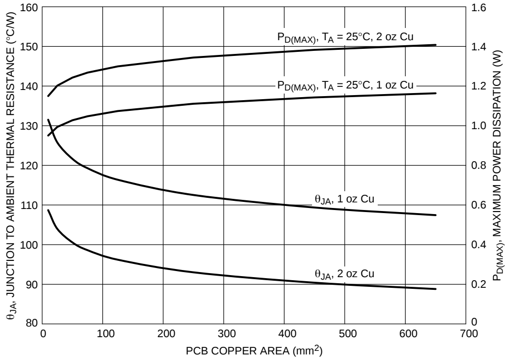
Figure 23. \theta_{JA} and P_{D(MAX)} vs. Copper Area (CSP4)
