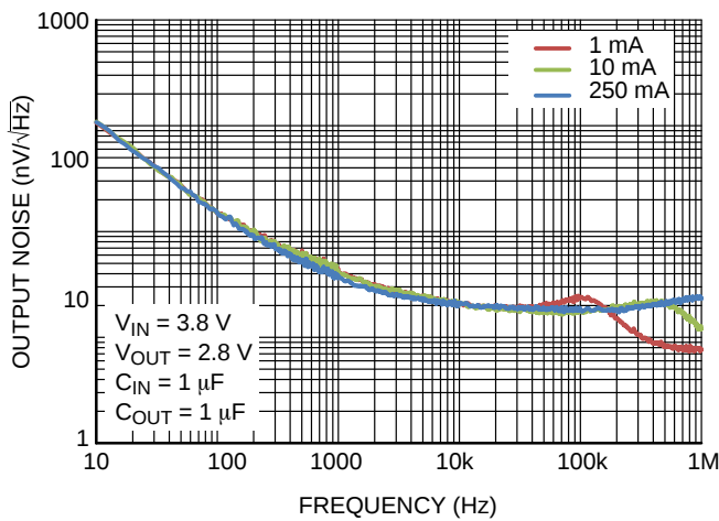
Figure 18. Output Voltage Noise Spectral Density – V_{OUT} = 2.8\text{ V}
