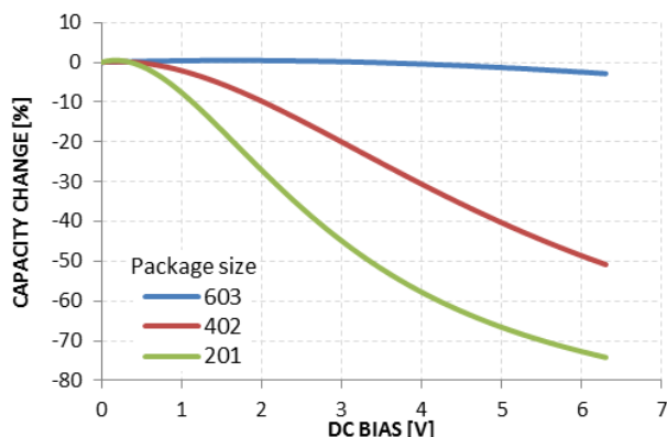
Figure 22. Capacity vs DC Bias Voltage
