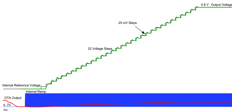
Figure 28. Soft-Start Details
