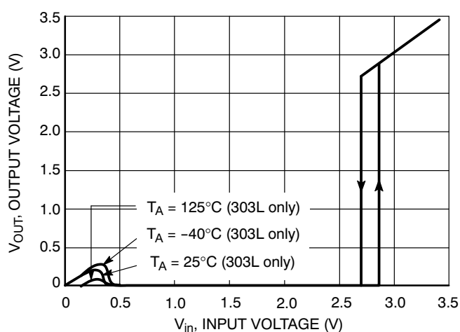
Figure 10. NCP302L/3L Series 2.7 V Reset Output Voltage vs. Input Voltage
