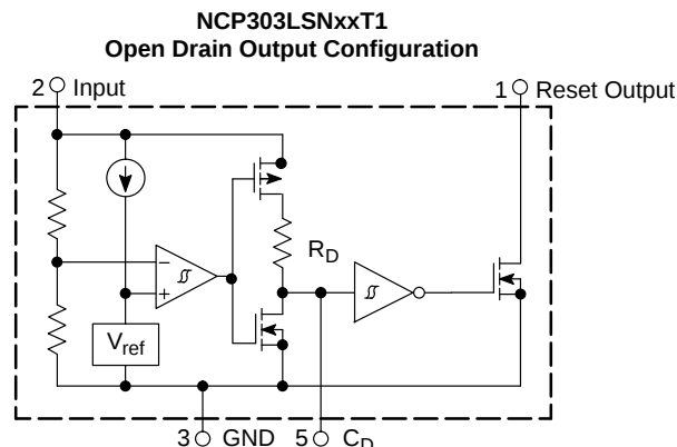
This device contains 28 active transistors. Figure 1. Representative Block Diagrams
