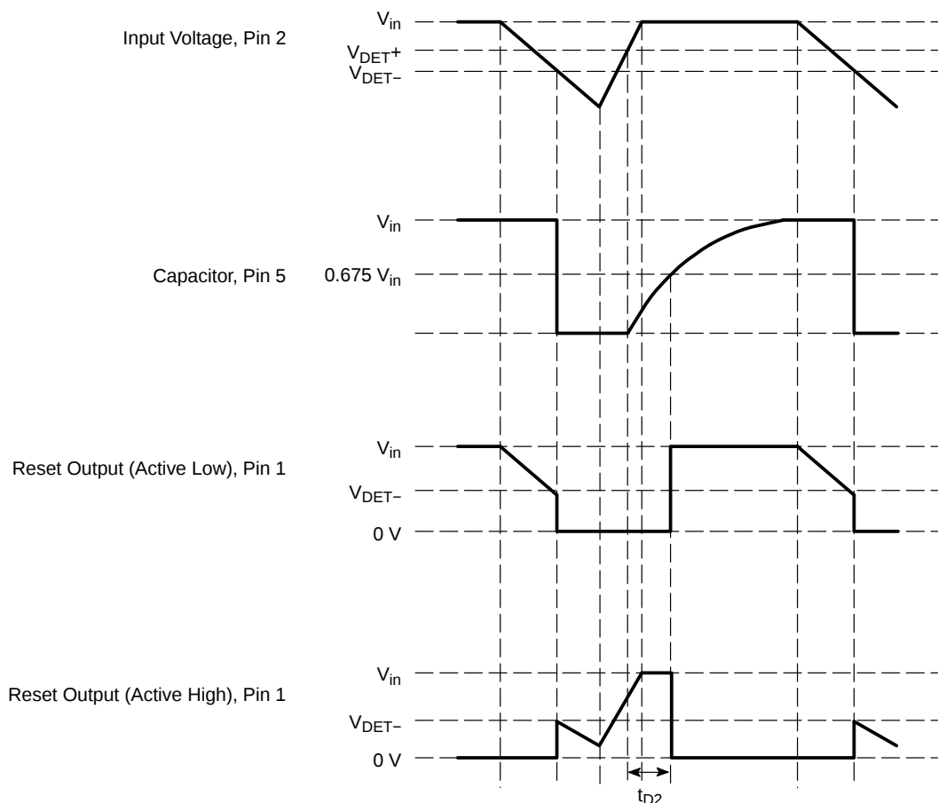
Figure 37. Timing Waveforms
