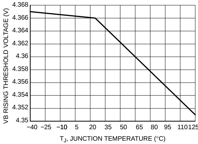
Figure 10. VB Rising Threshold Voltage vs. Junction Temperature
