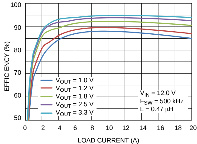
Figure 18. Efficiency vs. Load Current ( V_{IN} = 12.0\text{ V} ), Inductor: Würth Electronics 7443320047
