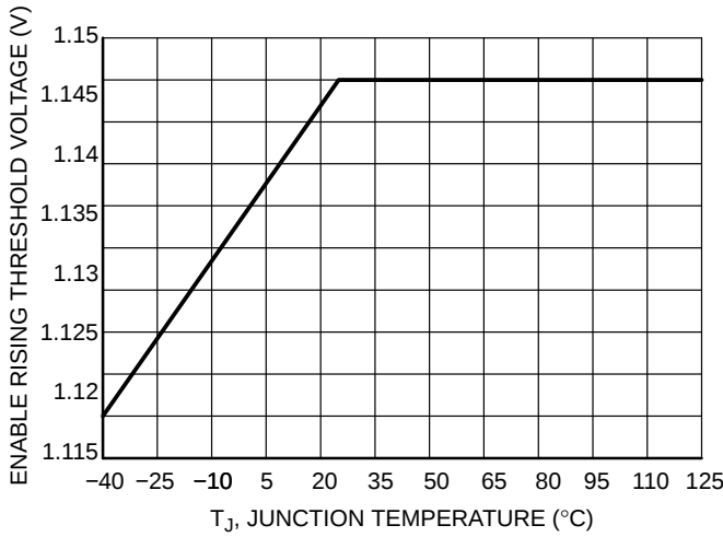
Figure 6. Enable Rising Threshold Voltage vs. Junction Temperature
