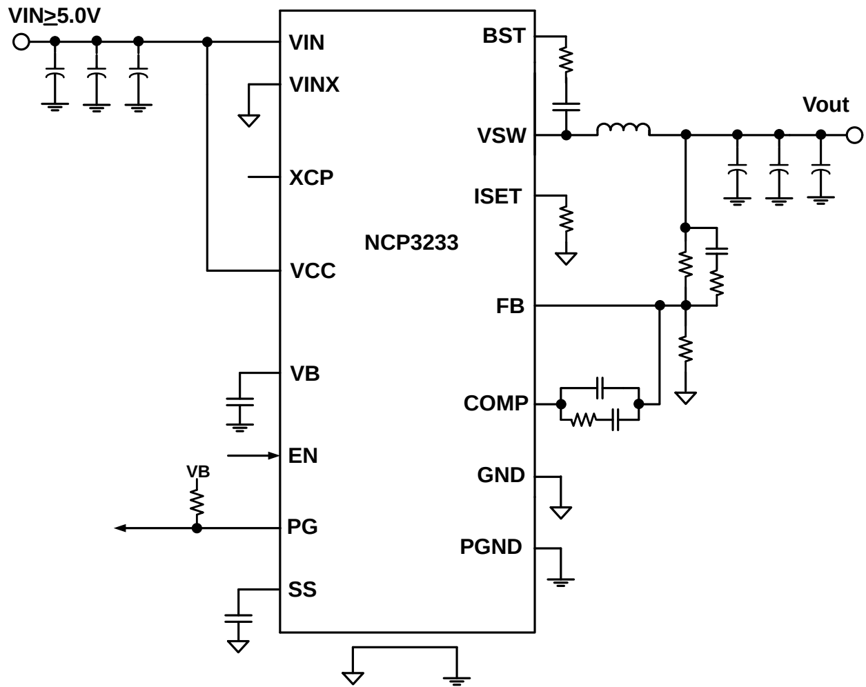
Figure 3. Typical Application Circuit for V_{IN} \geq 5.0V
