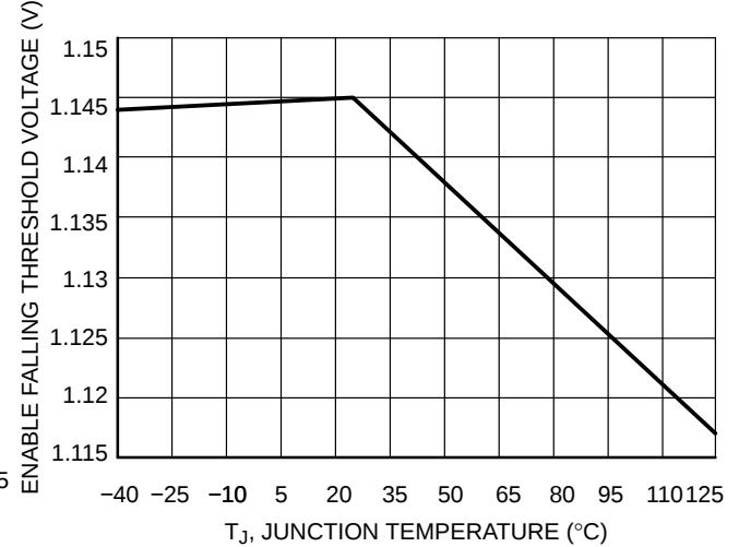
Figure 7. Enable Falling Threshold Voltage vs. Junction Temperature
