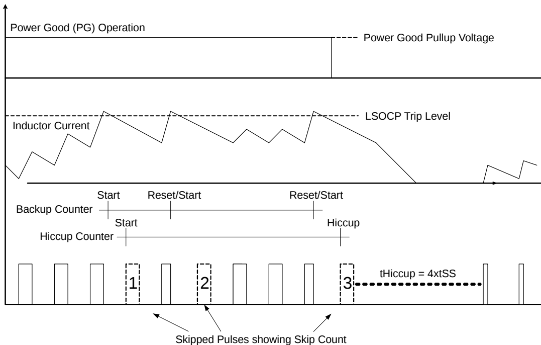
Figure 20. LSOCP Function with Counters and Power Good Shown (exaggerated for informational purposes)
