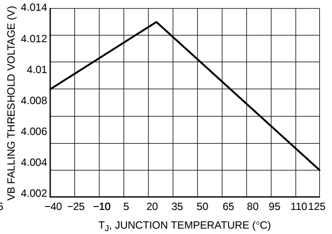
Figure 11. VB Falling Threshold Voltage vs. Junction Temperature
