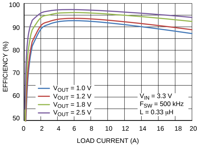
Figure 16. Efficiency vs. Load Current ( V_{IN} = 3.3\text{ V} ), Inductor: Würth Electronics 7443320033
