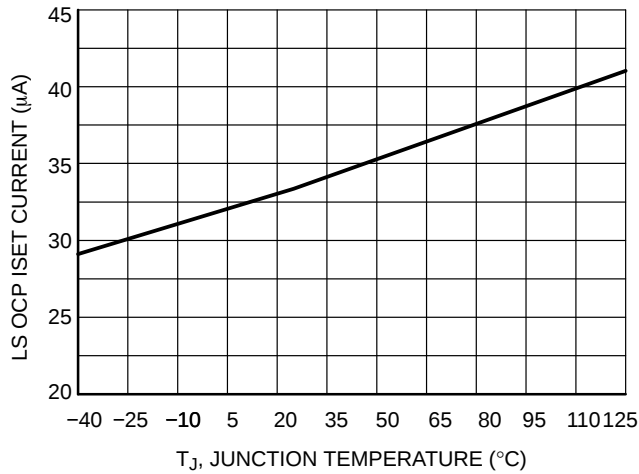
Figure 14. LS OCP ISET Current vs. Junction Temperature
