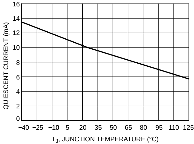
Figure 12. Quiescent Current vs. Junction Temperature (V CC = 12 V, No Switching)
