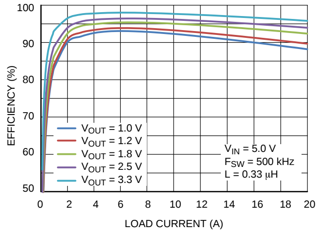
Figure 17. Efficiency vs. Load Current ( V_{IN} = 5.0\text{ V} ), Inductor: Würth Electronics 7443320033
