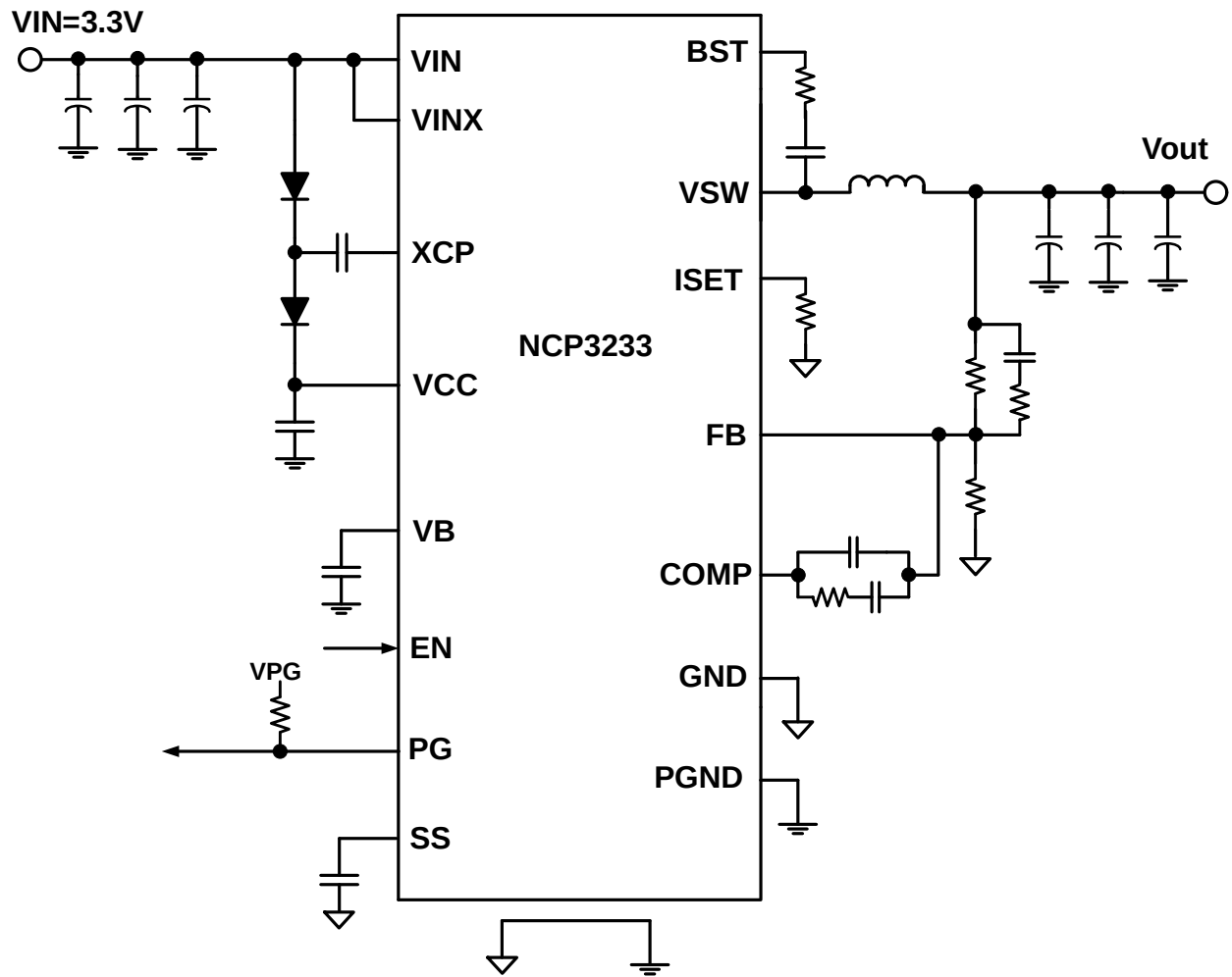
Figure 2. Typical Application Circuit for V_{IN} = 3.3\text{ V}
