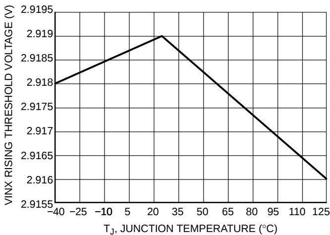
Figure 8. VINX Rising Threshold Voltage vs. Junction Temperature
