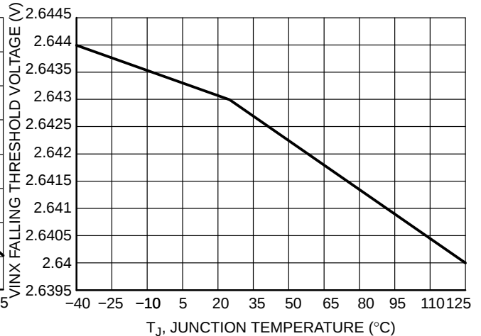
Figure 9. VINX Falling Threshold Voltage vs. Junction Temperature
