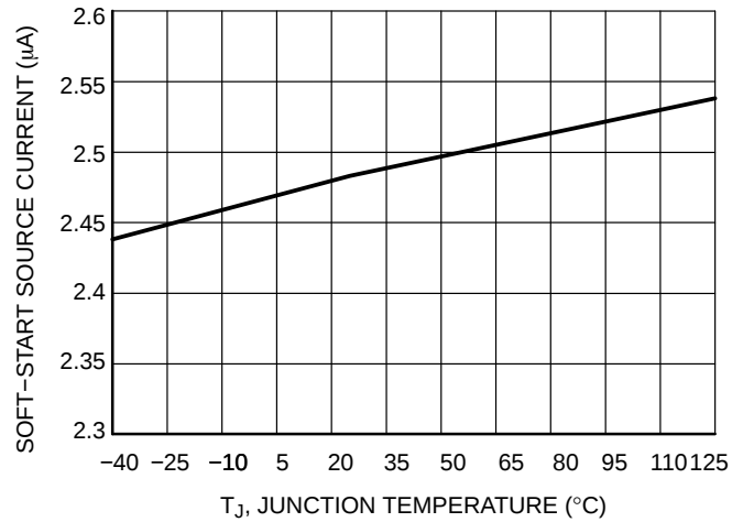
Figure 15. Soft-Source Current vs. Junction Temperature
