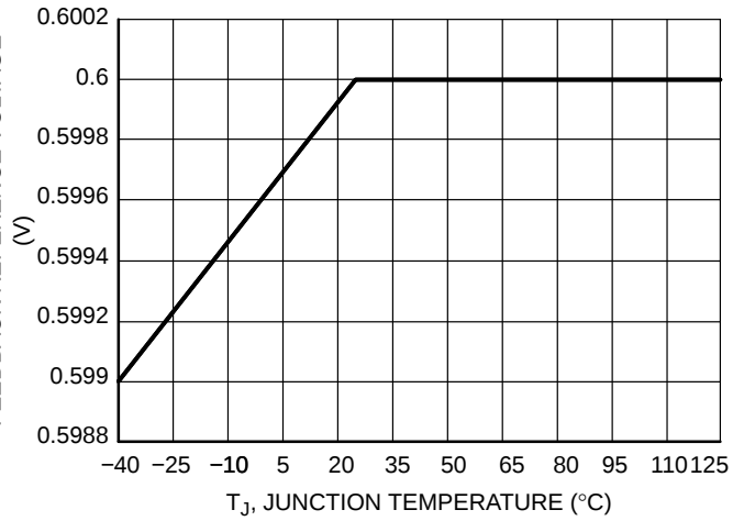
Figure 5. Feedback Reference Voltage vs. Junction Temperature (V IN = 4.5 V and 12 V)
