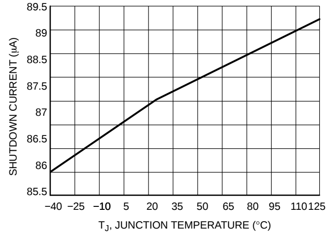
Figure 13. Shutdown Current vs. Junction Temperature (V IN = 12 V)
