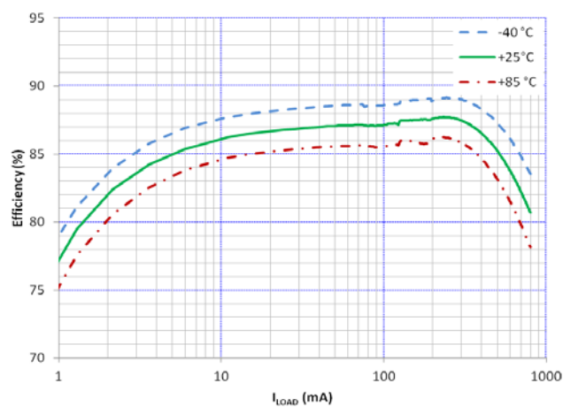
Figure 7. Efficiency vs I_{LOAD} and Temperature V_{OUT} = 1.20\text{ V} , SPM6530 Inductor
