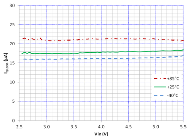
Figure 29. I_{Q\text{ LDO3}} vs V_{IN} and Temperature
