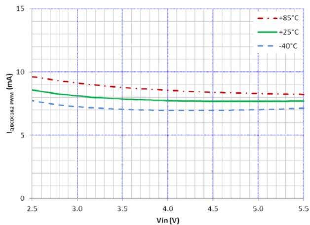
Figure 31. I_{Q\text{ PWM}} vs V_{IN} and Temperature
