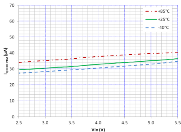
Figure 30. I_{Q\text{ PFM}} vs V_{IN} and Temperature
