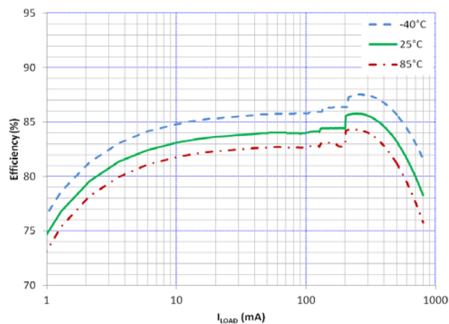
Figure 13. Efficiency vs I_{LOAD} and Temperature DCDC2, V_{OUT} = 1.20\text{ V} , SPM3012 Inductor
