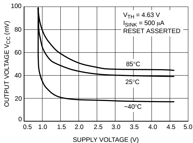
Figure 7. Output Voltage Low vs. Supply Voltage
