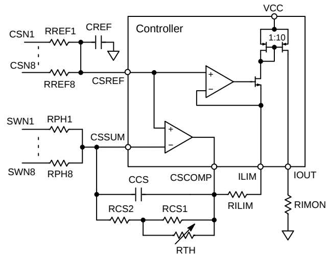
Figure 8. Total Current Summing Amplifier
