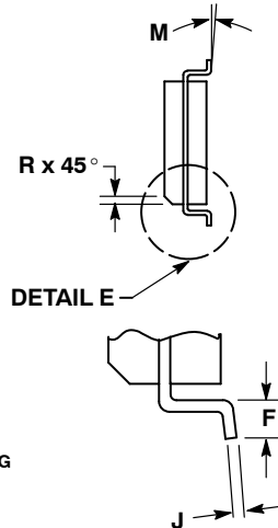
DETAIL E
