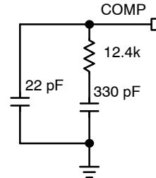
Figure 32. Recommended Compensation for Primary Switcher
