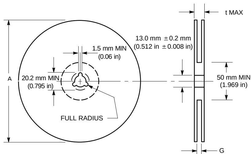
Figure 26. Reel Dimensions
