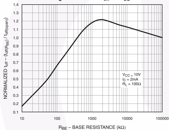
Fig. 9 Normalized t_{\text{off}} vs. R_{\text{BE}}
