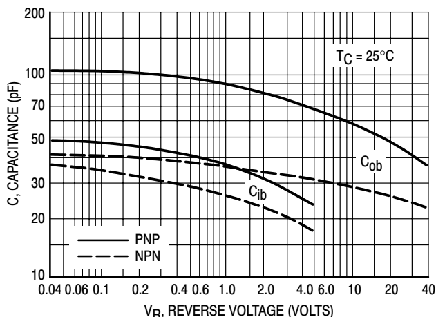
Figure 7. Capacitance
