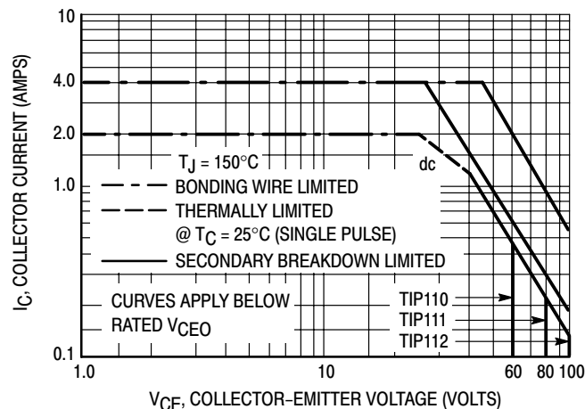
Figure 6. TIP110, 111, 112
