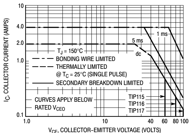
Figure 6. TIP115, 116, 117
