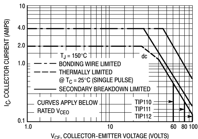
Figure 7. TIP110, 111, 112
