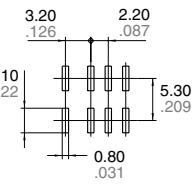
Suggested mounting pad
