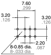
PC board pattern
