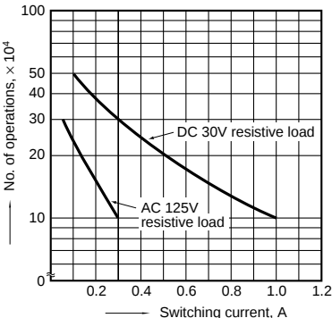
2. Life curve
