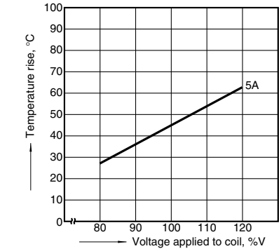
2.-(1) Coil temperature rise (1 Form C AC type) Measured portion: Inside the coil Ambient temperature: 30°C 86°F
