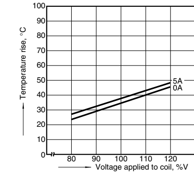
2.-(4) Coil temperature rise (1 Form C DC type) Measured portion: Inside the coil Ambient temperature: 30°C 86°F
