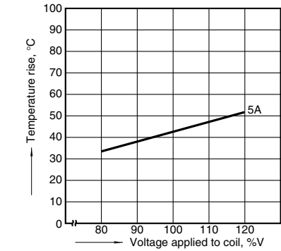
2.-(5) Coil temperature rise (2 Form C DC type) Measured portion: Inside the coil Ambient temperature: 30°C 86°F
