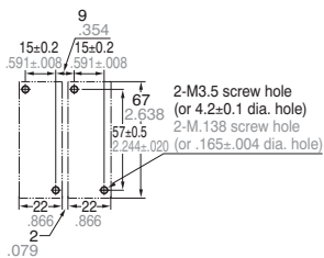
Mounting hole diagram HC2-Slim type
