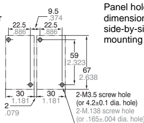
HC vertical type
