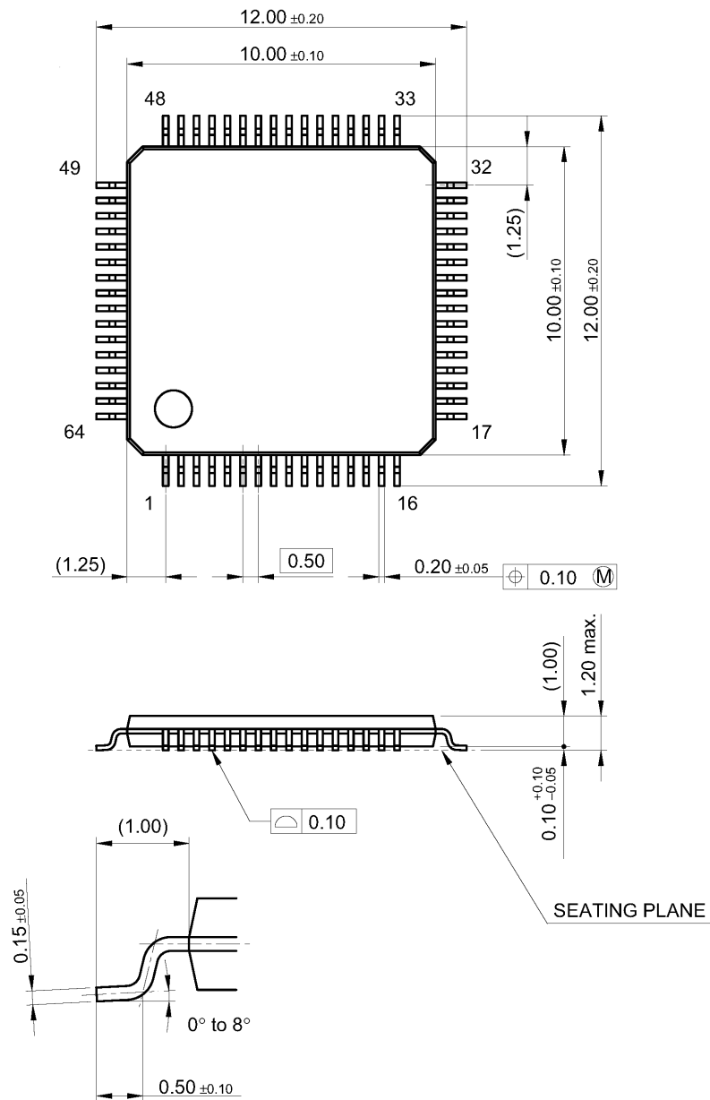
Figure:1.6.2 64-pin TQFP Package Dimension
