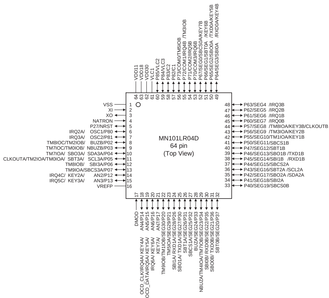
Figure:1.4.2 MN101LR04D Pin Configuration
