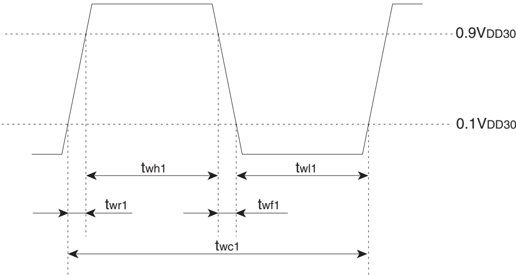
Figure:1.5.3 OSC1 timing diagram
