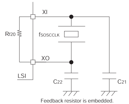
Figure:1.5.2 Low-speed oscillation
