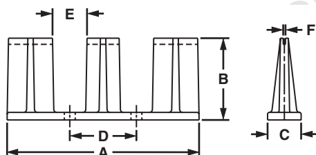
High Holder (FSHH-X)
