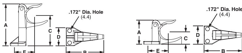
CPH Corner Post, High
