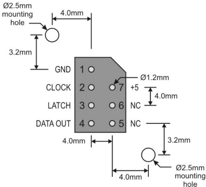
NES Socket pin out
