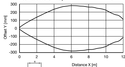
Movement Characteristics (aperture ML17-OA-10V mounted at transmitter)
