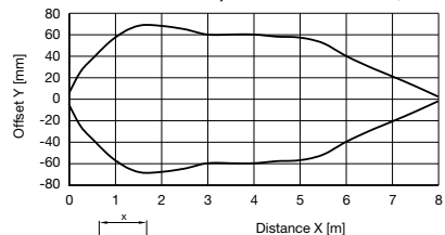
Movement Characteristics (aperture ML17-OA-05V mounted at transmitter)
