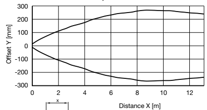
Movement Characteristics (aperture ML17-OA-25V mounted at transmitter)
