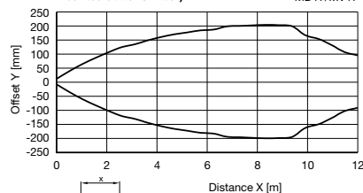
Movement Characteristics (aperture ML17-OA-25H mounted at transmitter)
