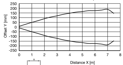
Movement Characteristics (aperture ML17-OA-25V mounted at both transmitter and receiver)
