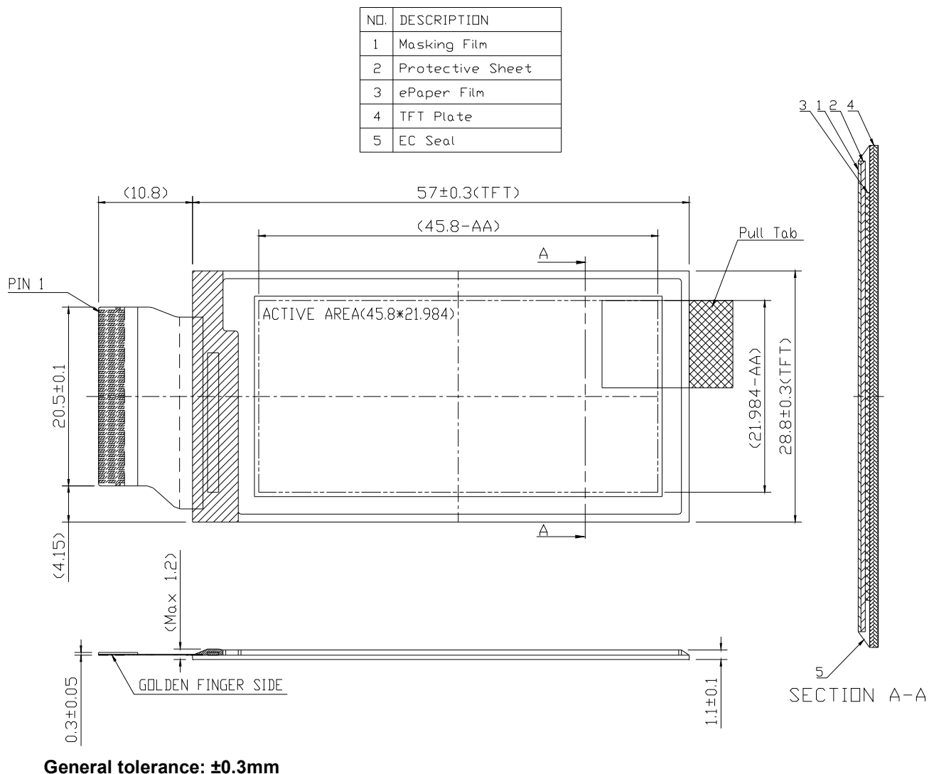
Figure 1-1 EPD Drawing
