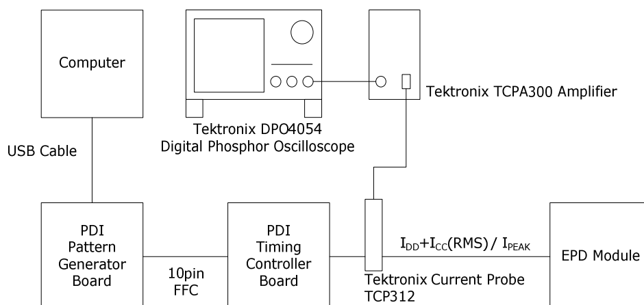
Figure 3-3 Current Measurement
