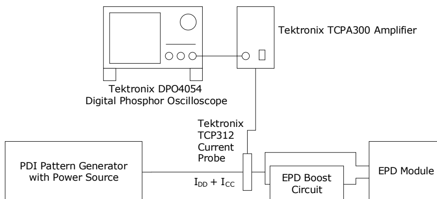
Figure 3-3 Current Measurement
