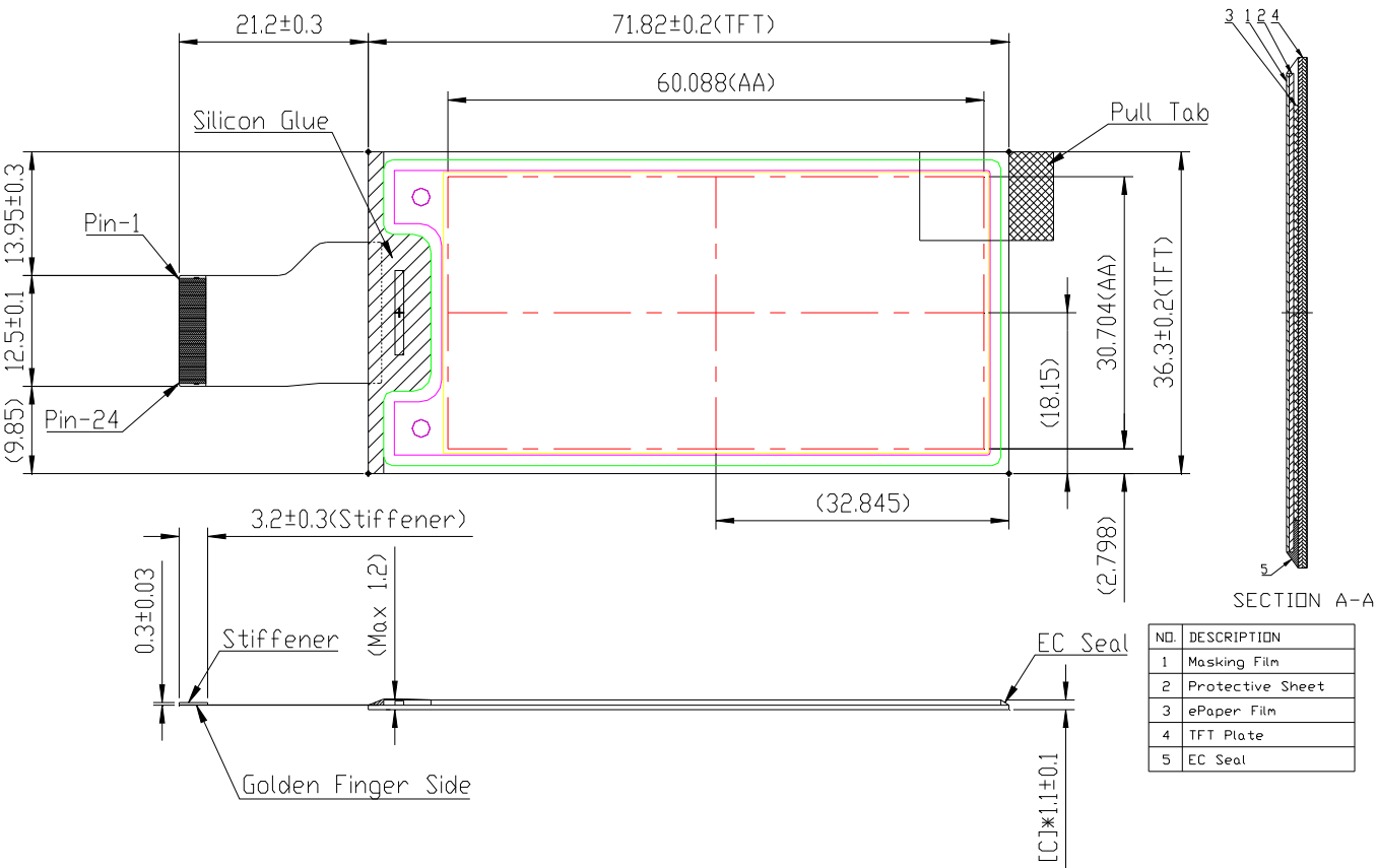
Figure 1-1EPD Drawing
