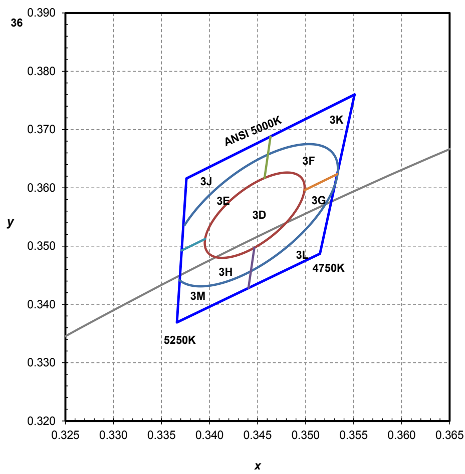
Figure 16. 5000K 1/9 th color bin structure.
