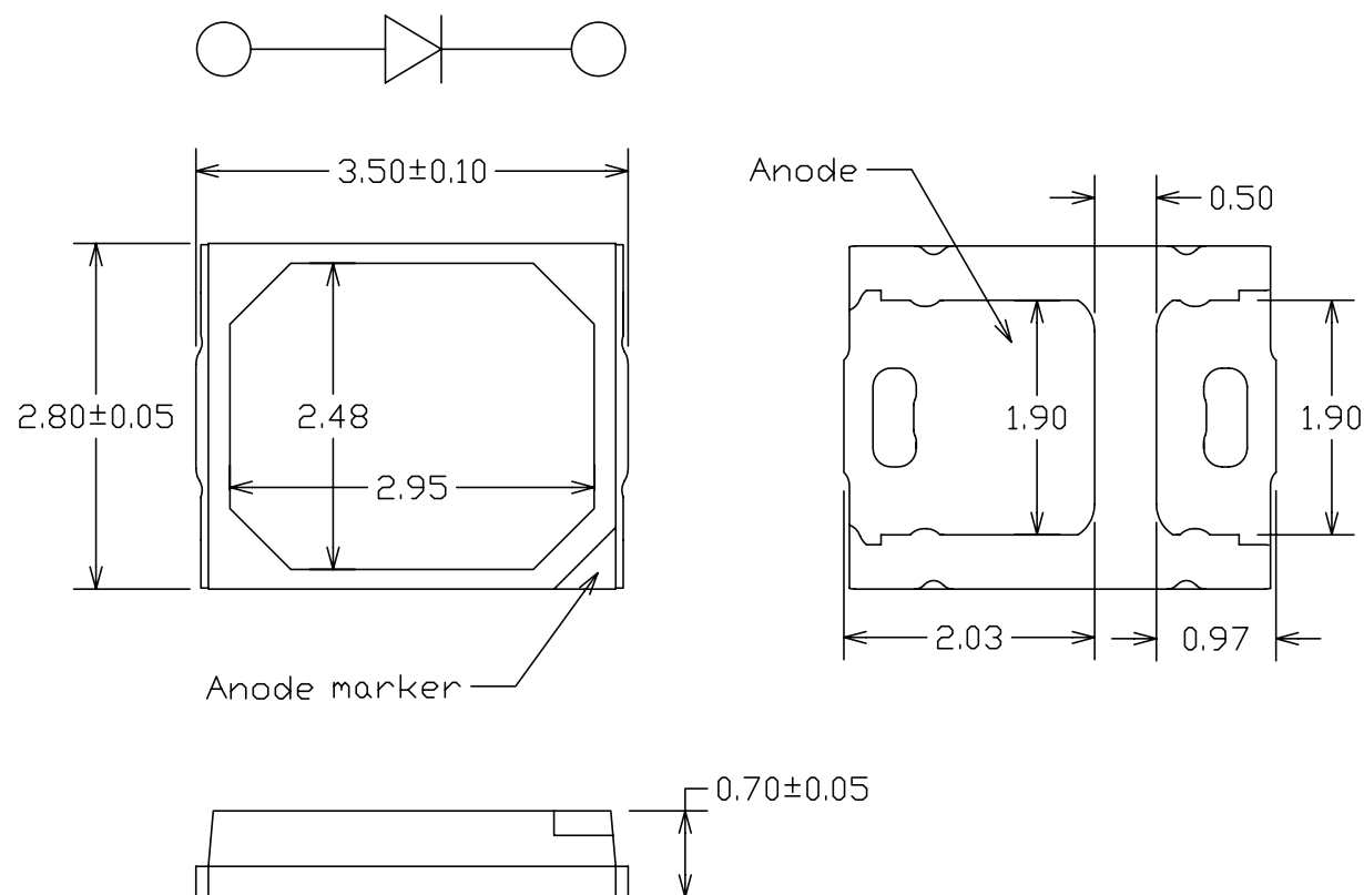
Figure 6. Mechanical dimensions for LUXEON SunPlus 2835 Line.
