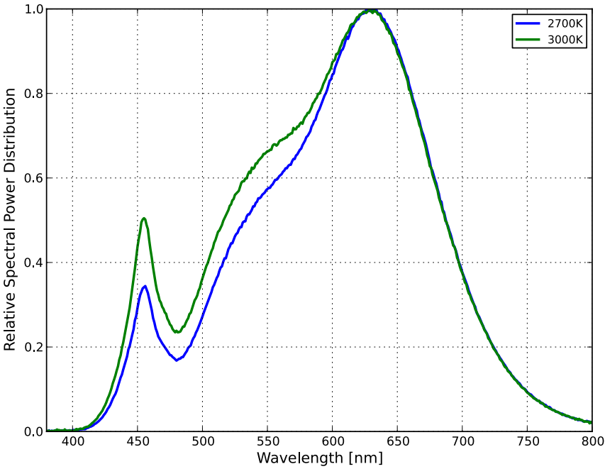
Figure 6. Color Spectrum of L1T2-xx900000000000.
