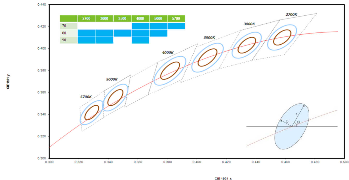
Figure 7. 3-step and 5-step MacAdam ellipse color bins.
