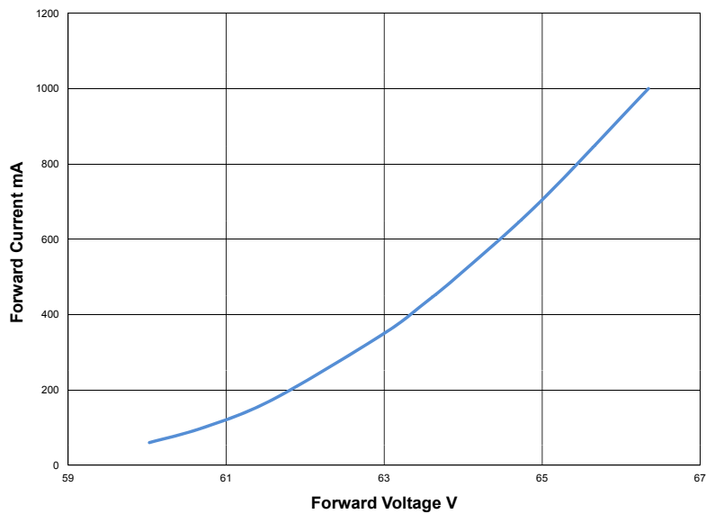
Figure 13. Forward current vs. forward voltage for L XK8-PW27-0024, L XK8-PW30-0024, L XK8-PW35-0024, L XK8-PW40-0024, L XK8-PW50-0024 24-up products.
