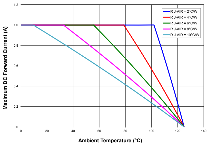
Figure 15. Maximum forward current vs. ambient temperature, based on T_{JMAX} = 125^{\circ}\text{C} .
