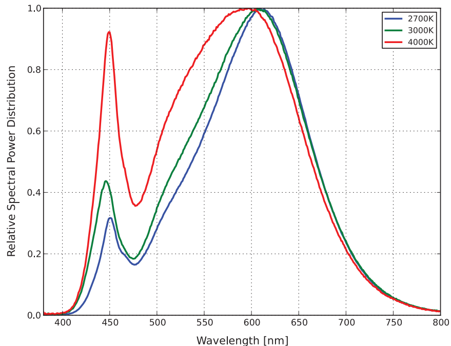
Figure 6. Color spectrum of LXK8-PW27-xxxx product, integrated measurement.
