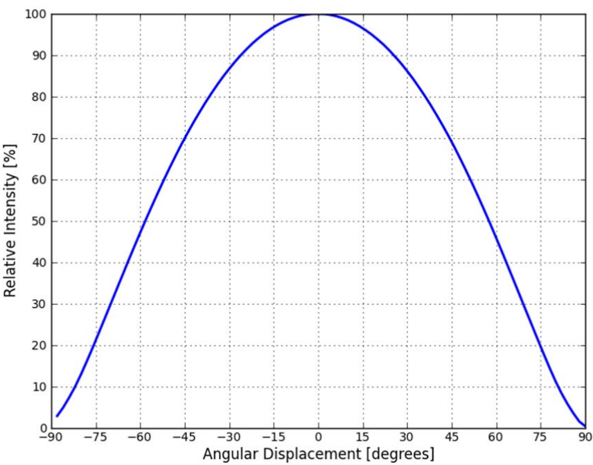
Figure 9. Radiation pattern for MXZx-PWxx.
