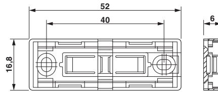
Dimensioned drawing
