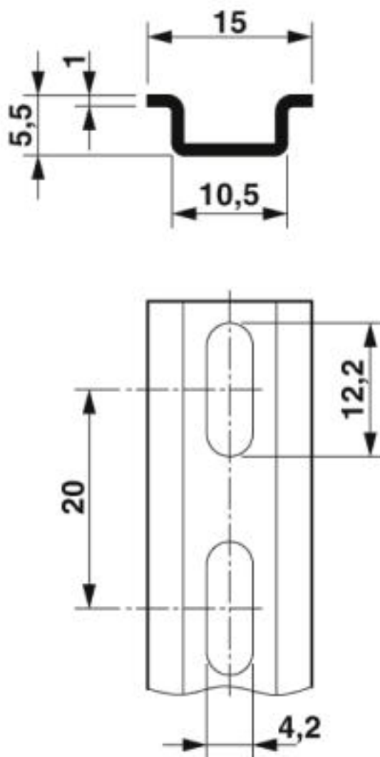
Dimensional drawing
