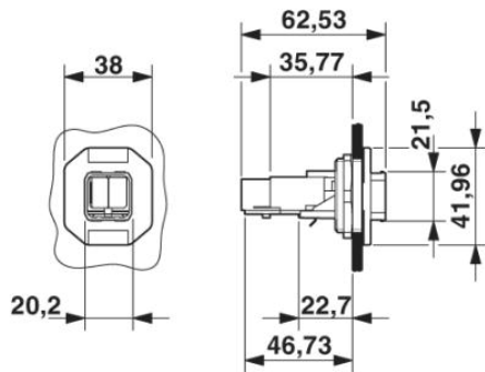
Push-Pull SCRJ panel mounting frame
