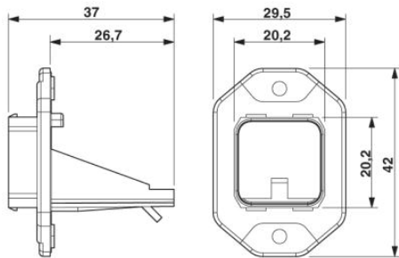
Push-Pull panel mounting frame, Freetnet system, IP67
