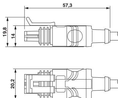
Superseal, socket, view from above and side
