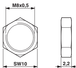
Dimensioned drawing
