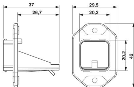
Push-Pull panel mounting frame, Freenet system, IP67
