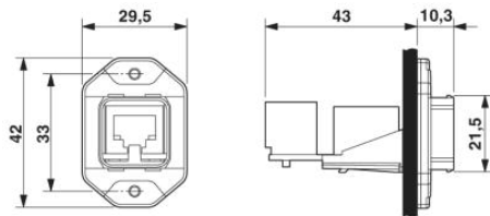
Push-Pull SCRJ panel mounting frame
