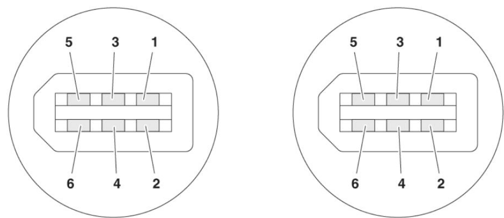
Pin assignment plug FireWire
